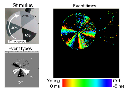
DVS in use: events from a spinning angle grinder recorded at microsecond precision
